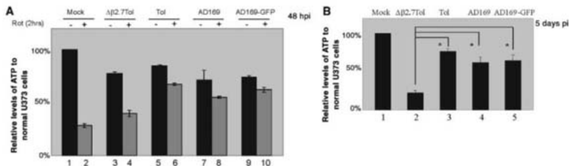
Fig. 3. \beta 2.7 expression maintains ATP production in infected cells. (A) Percentage of ATP content of mock- (1 and 2), \Delta\beta 2.7 Tol- (3 and 4), Toledo- (5 and 6), AD169-, and AD169-GFP-infected cells with (2, 4, 6, 8, and 10) or without (1, 3, 5, 7, and 9) rotenone for 2 hours was determined at 48 hpi, as compared to mock (1).
